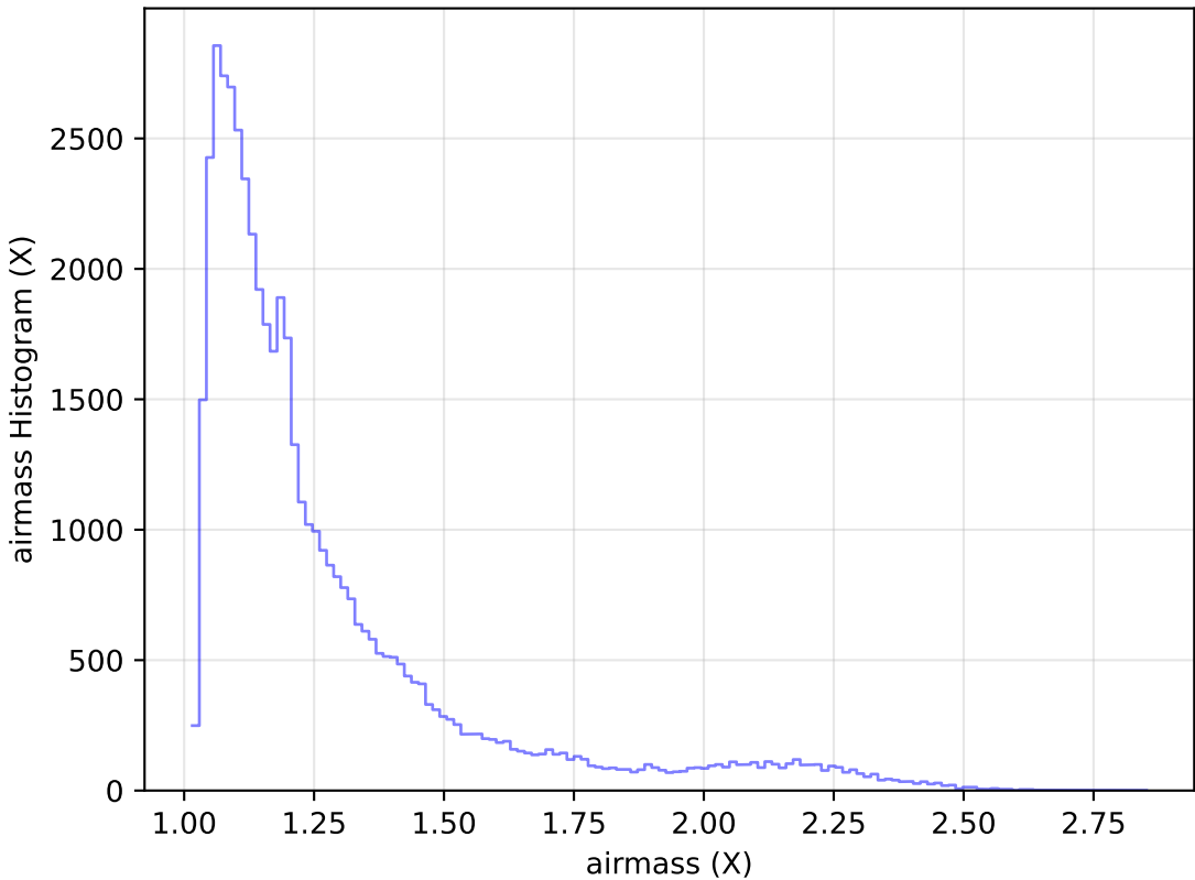
too_elab_r32_d3_gz_v3.4_10yrs Yr 1 r band: airmass Histogram
