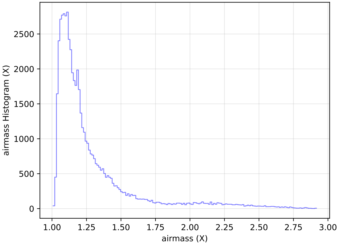
too_elab_r32_d3_gz_v3.4_10yrs Yr 1 i band: airmass Histogram
