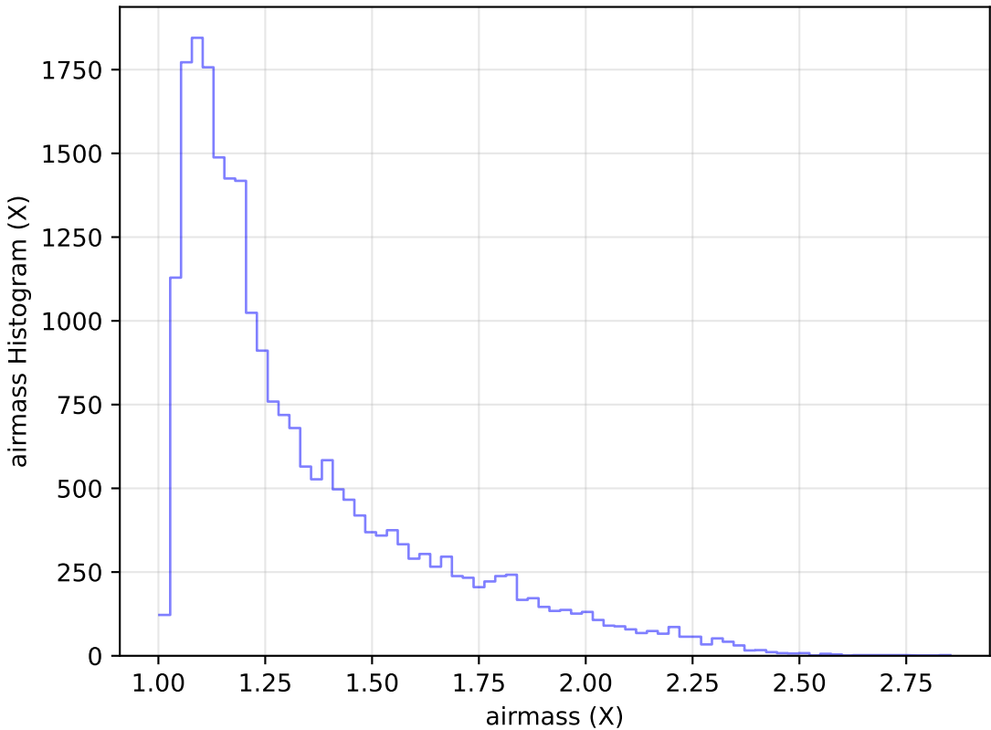
too_elab_r32_d3_gz_v3.4_10yrs Yr 1 g band: airmass Histogram
