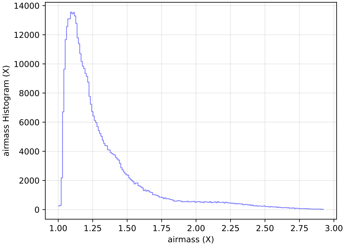
too_elab_r32_d3_gz_v3.4_10yrs WFD z band: airmass Histogram
