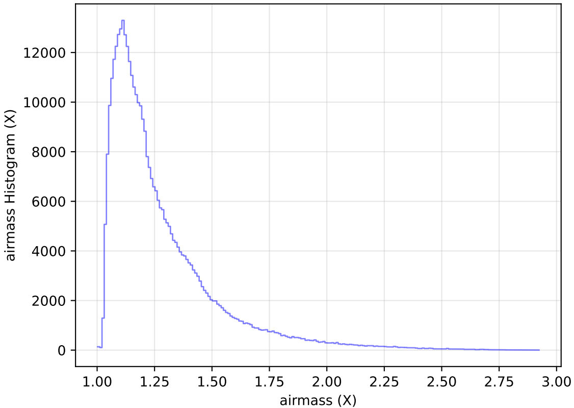
too_elab_r32_d3_gz_v3.4_10yrs WFD y band: airmass Histogram
