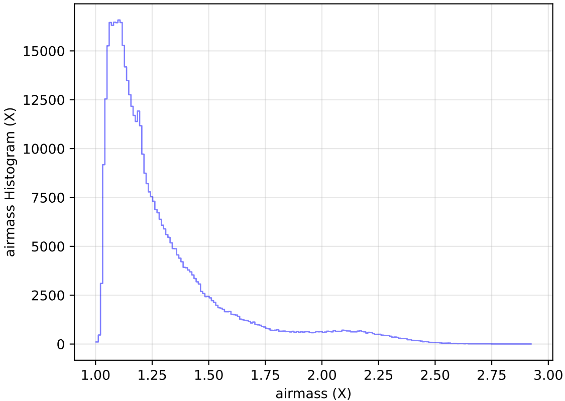
too_elab_r32_d3_gz_v3.4_10yrs WFD r band: airmass Histogram
