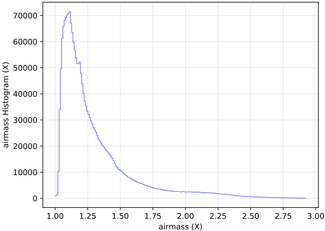
too_elab_r32_d3_gz_v3.4_10yrs WFD all bands: airmass Histogram
