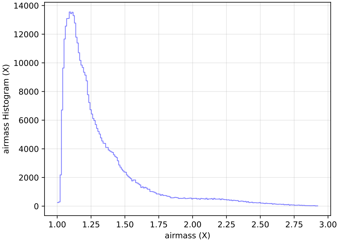
too_elab_r32_d3_gz_v3.4_10yrs All sky z band: airmass Histogram
