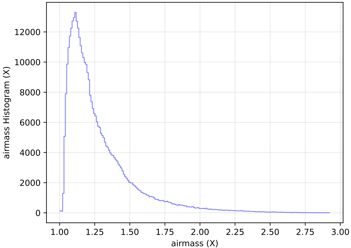
too_elab_r32_d3_gz_v3.4_10yrs All sky y band: airmass Histogram
