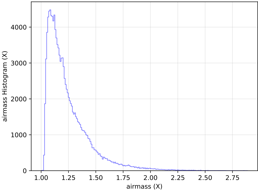
too_elab_r32_d3_gz_v3.4_10yrs All sky u band: airmass Histogram
