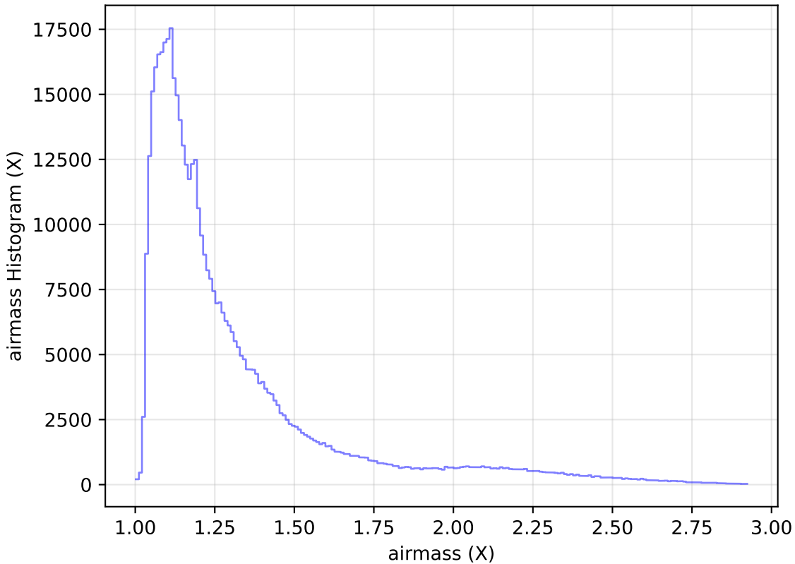
too_elab_r32_d3_gz_v3.4_10yrs All sky i band: airmass Histogram
