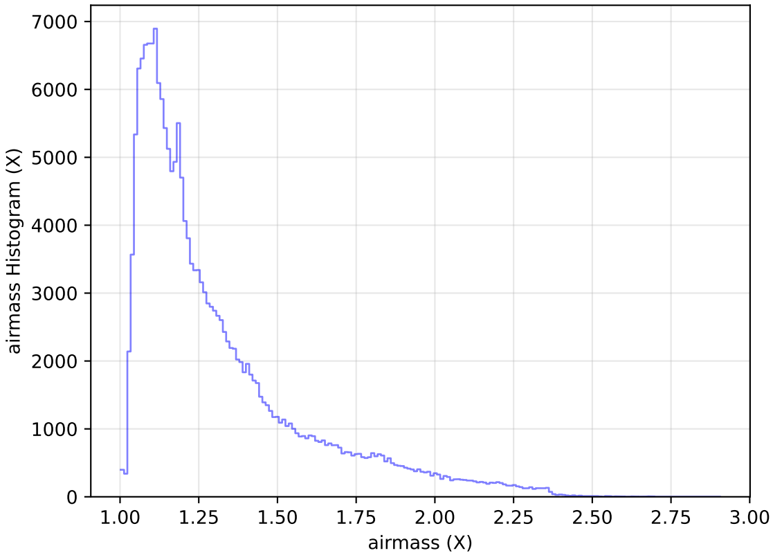
too_elab_r32_d3_gz_v3.4_10yrs All sky g band: airmass Histogram
