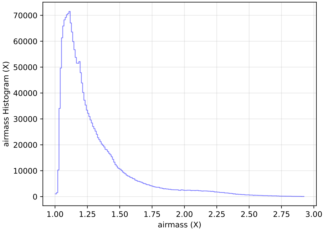
too_elab_r32_d3_gz_v3.4_10yrs All sky all bands: airmass Histogram
