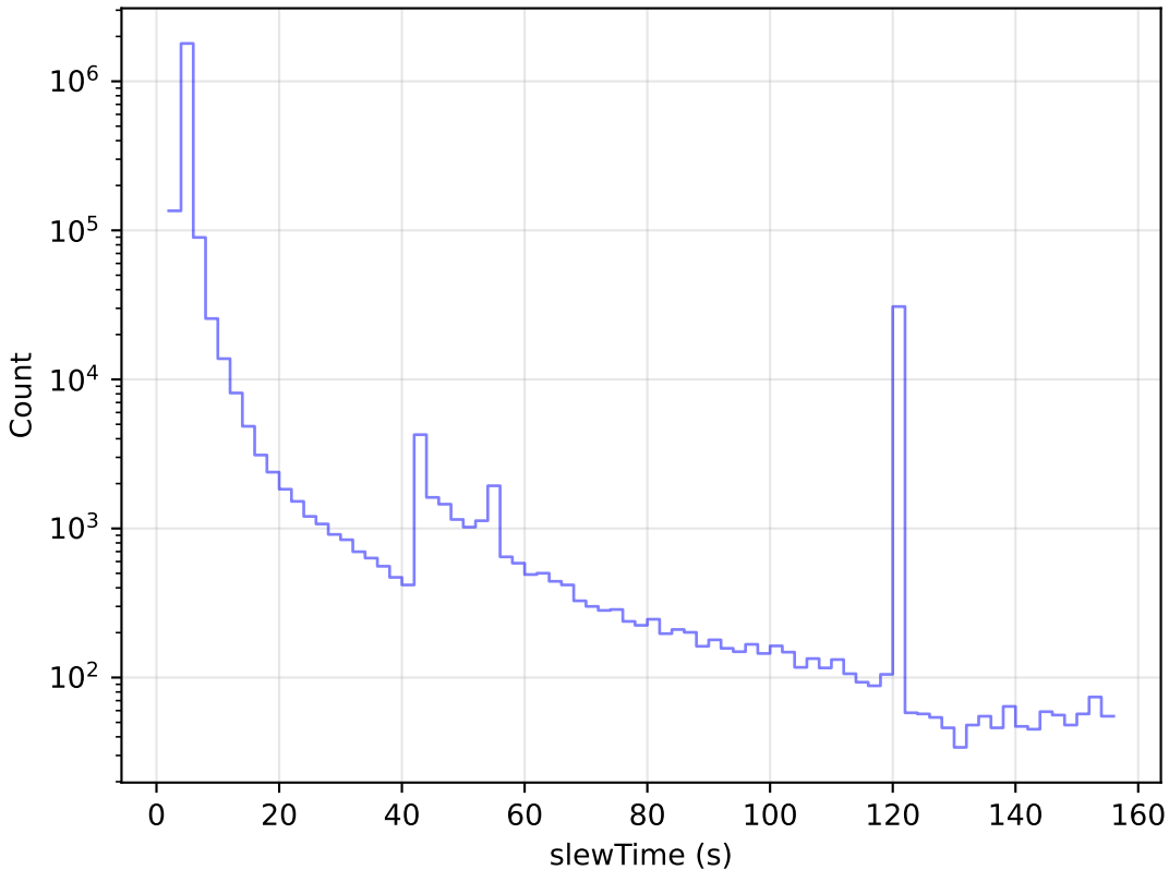
too_elab_r32_d3_gz_v3.4_10yrs All visits: Slew Time Histogram
