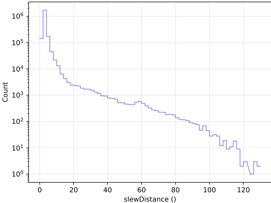
too_elab_r32_d3_gz_v3.4_10yrs All visits: Slew Distance Histogram
