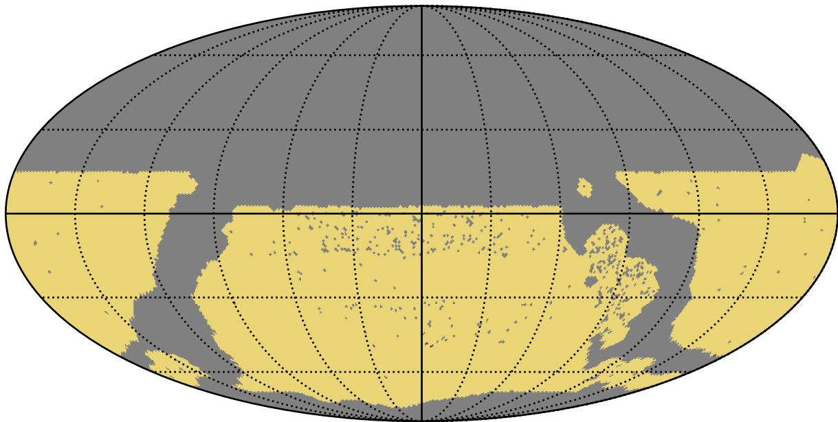
too_elab_r32_d3_gz_v3.4_10yrs WFD: RapidRevisits
