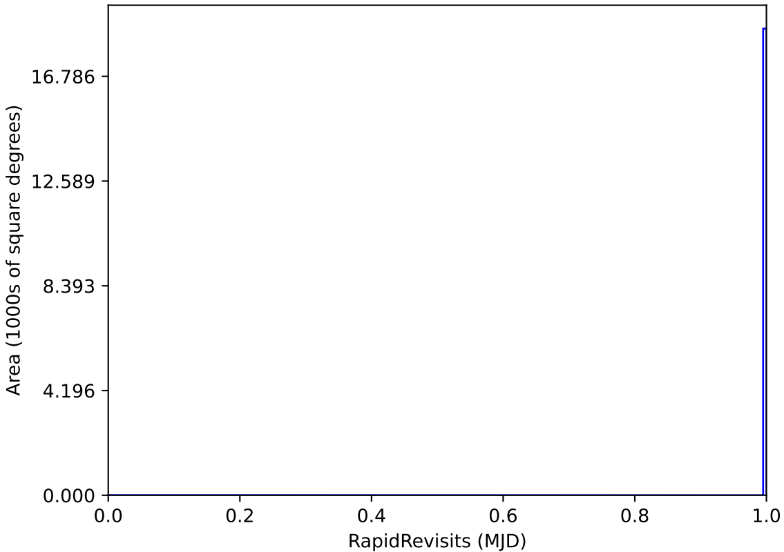
too_elab_r32_d3_gz_v3.4_10yrs WFD: RapidRevisits
