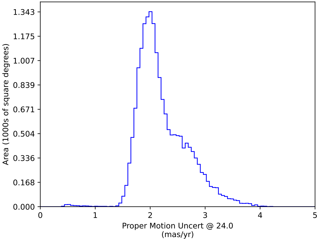
too_elab_r32_d3_gz_v3.4_10yrs WFD: Proper Motion Uncert @ 24.0
