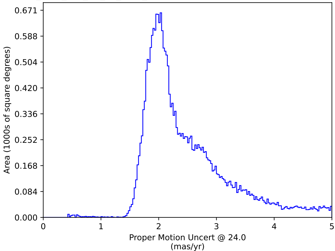
too_elab_r32_d3_gz_v3.4_10yrs All sky: Proper Motion Uncert @ 24.0
