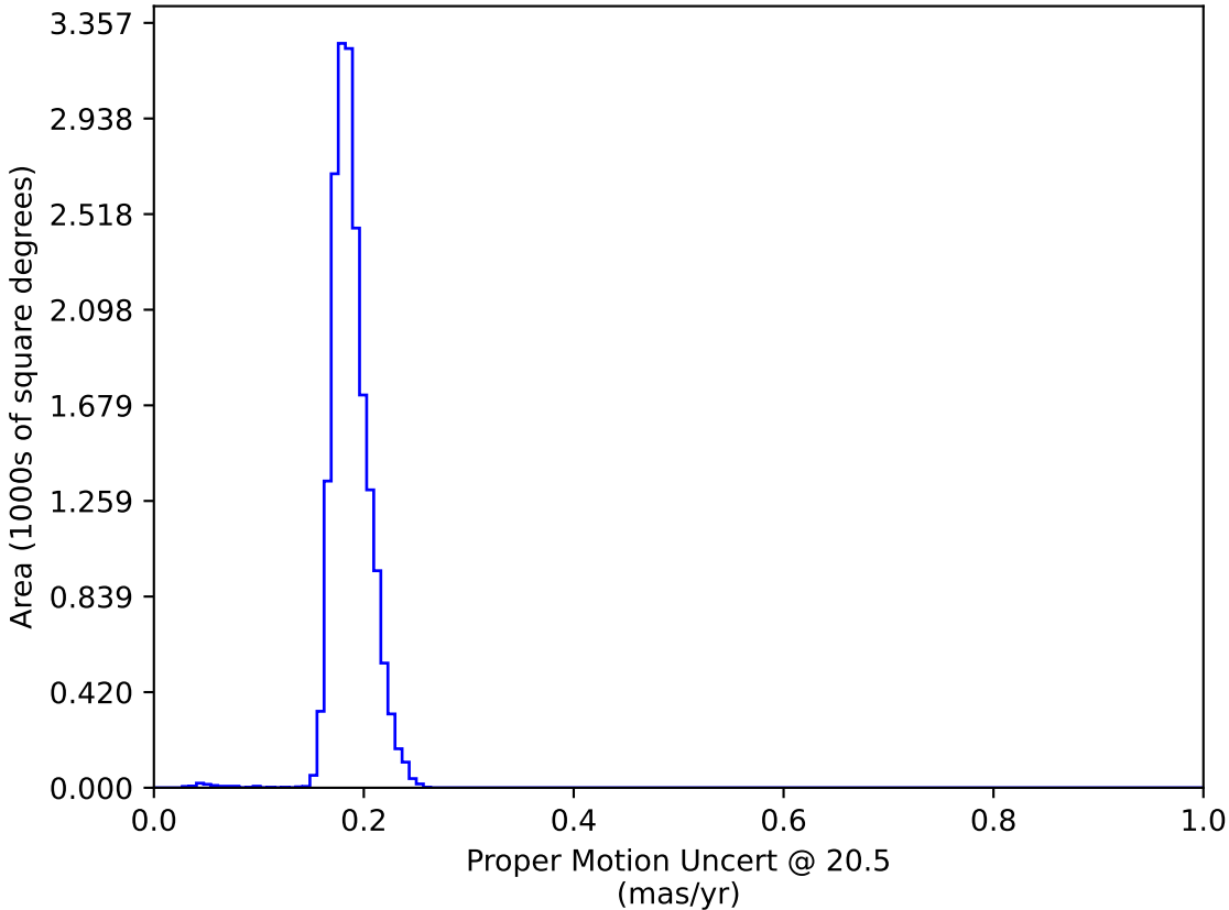
too_elab_r32_d3_gz_v3.4_10yrs WFD: Proper Motion Uncert @ 20.5
