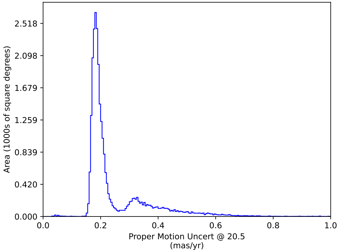
too_elab_r32_d3_gz_v3.4_10yrs All sky: Proper Motion Uncert @ 20.5
