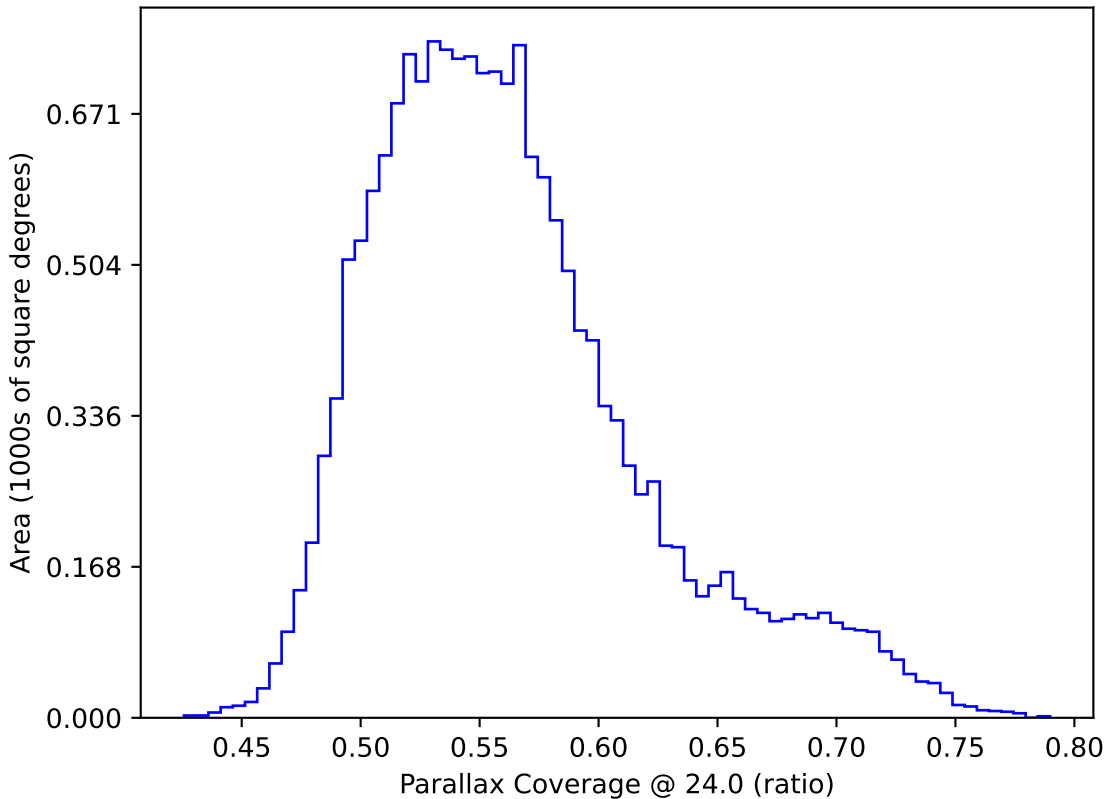
too_elab_r32_d3_gz_v3.4_10yrs WFD: Parallax Coverage @ 24.0
