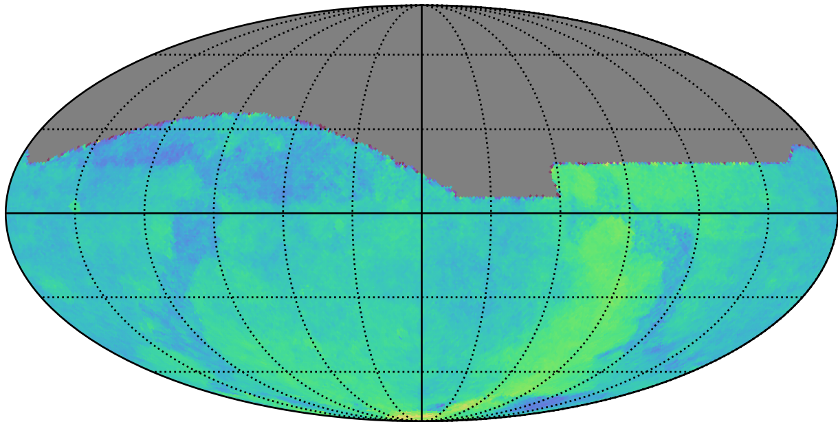
too_elab_r32_d3_gz_v3.4_10yrs All sky: Parallax Coverage @ 24.0
