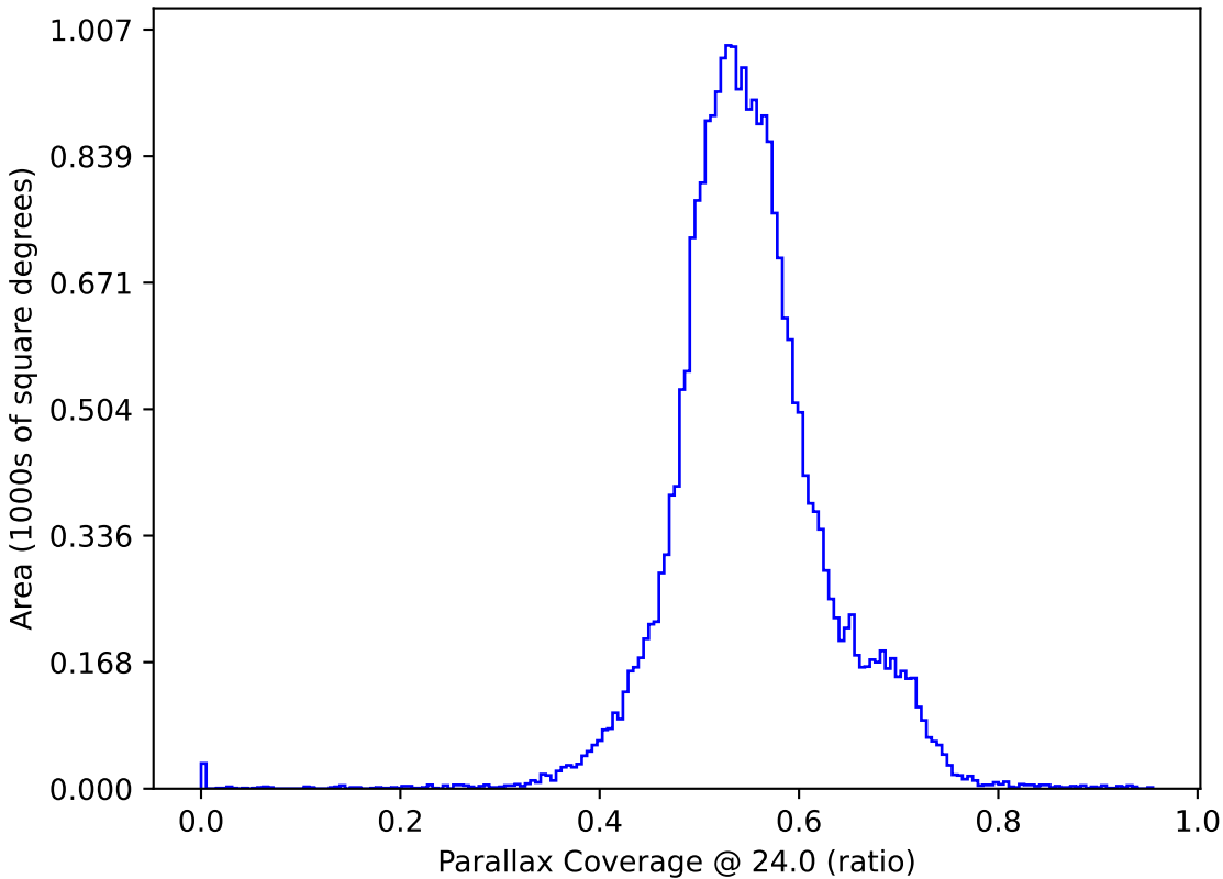
too_elab_r32_d3_gz_v3.4_10yrs All sky: Parallax Coverage @ 24.0
