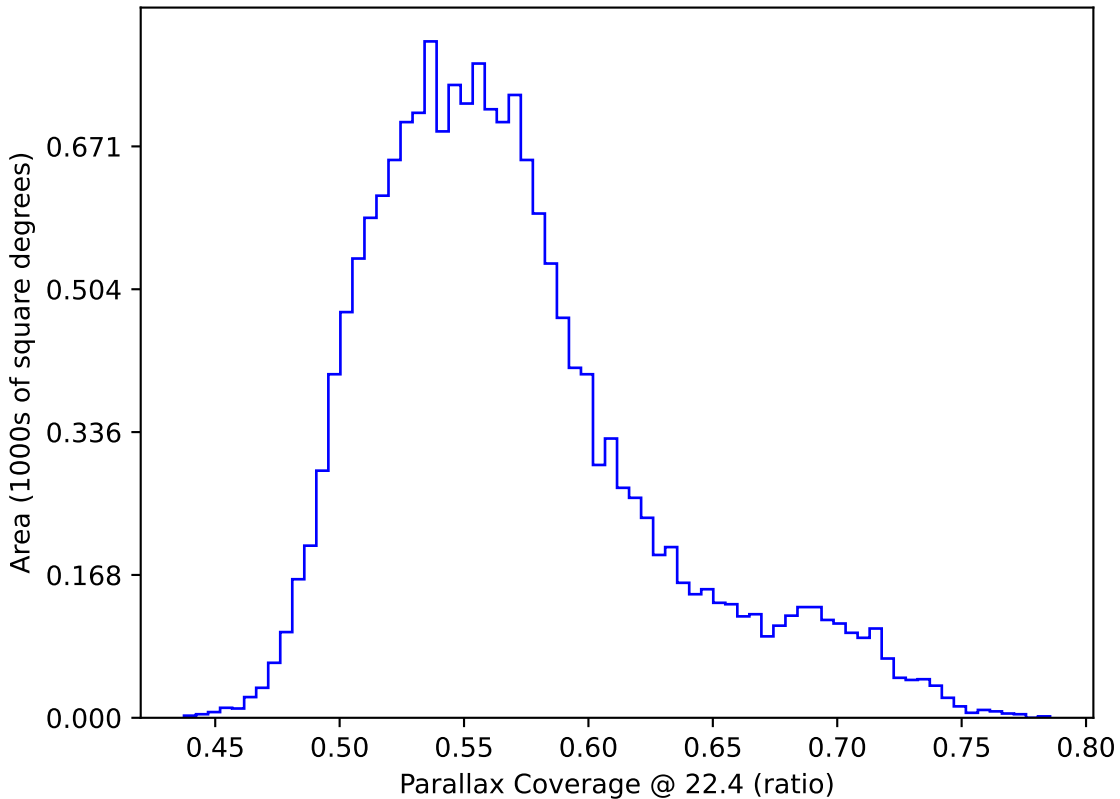
too_elab_r32_d3_gz_v3.4_10yrs WFD: Parallax Coverage @ 22.4
