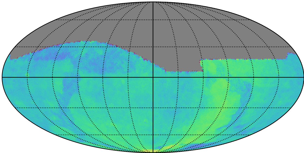
too_elab_r32_d3_gz_v3.4_10yrs All sky: Parallax Coverage @ 22.4
