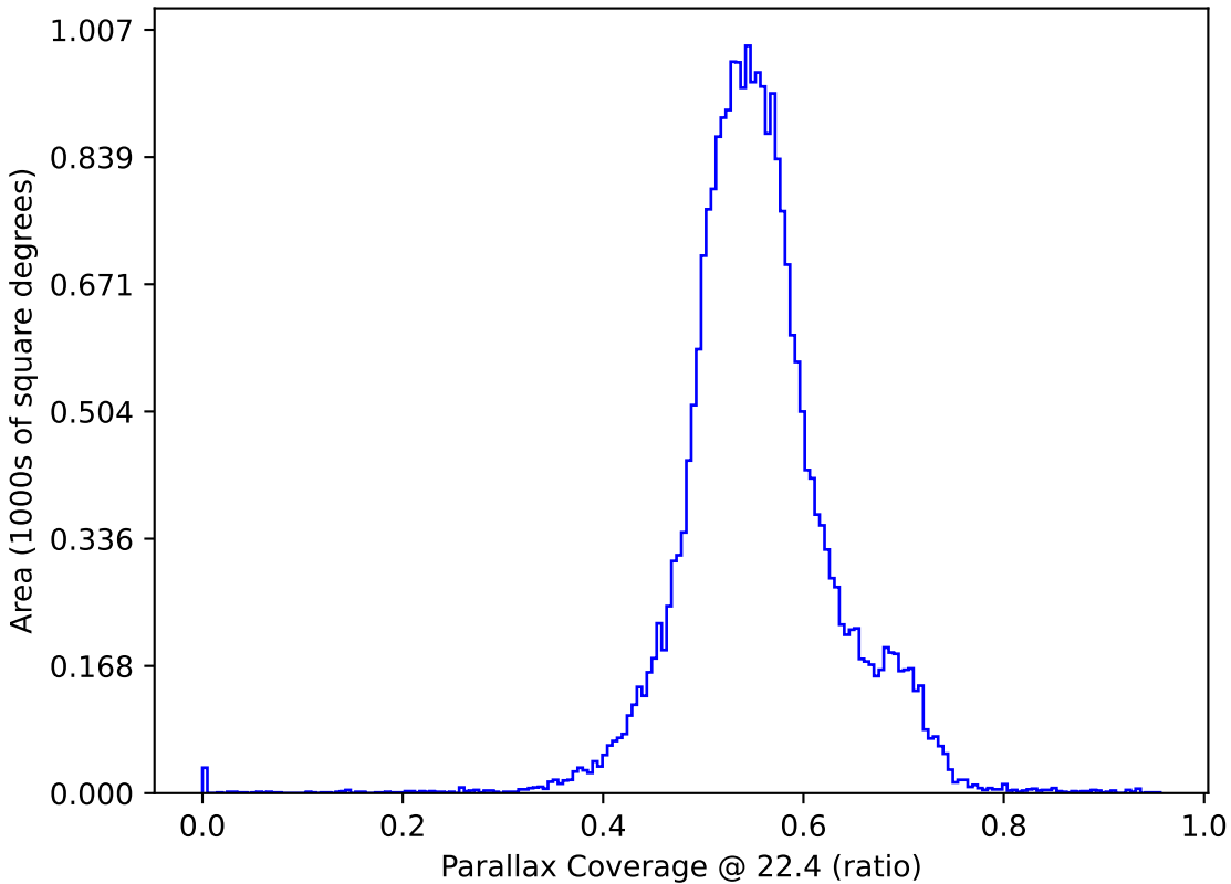
too_elab_r32_d3_gz_v3.4_10yrs All sky: Parallax Coverage @ 22.4
