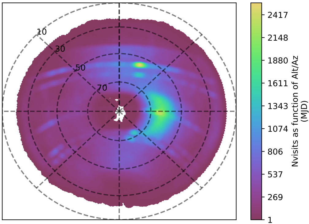
too_elab_r32_d3_gz_v3.4_10yrs z band: Nvisits as function of Alt/Az
