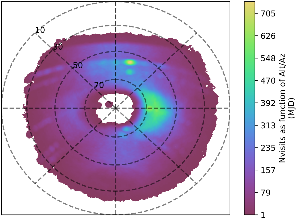
too_elab_r32_d3_gz_v3.4_10yrs u band: Nvisits as function of Alt/Az
