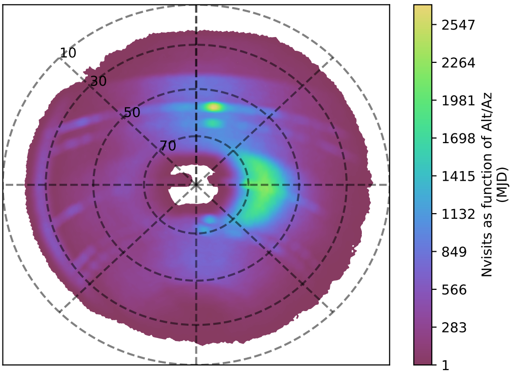
too_elab_r32_d3_gz_v3.4_10yrs r band: Nvisits as function of Alt/Az
