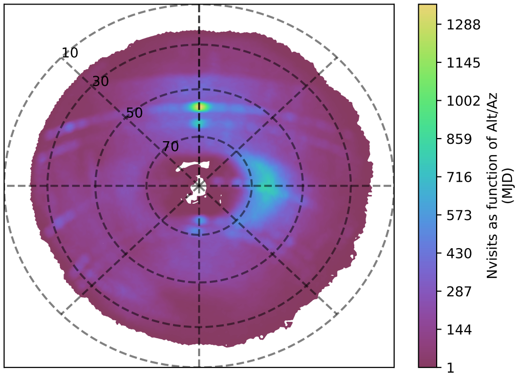
too_elab_r32_d3_gz_v3.4_10yrs g band: Nvisits as function of Alt/Az
