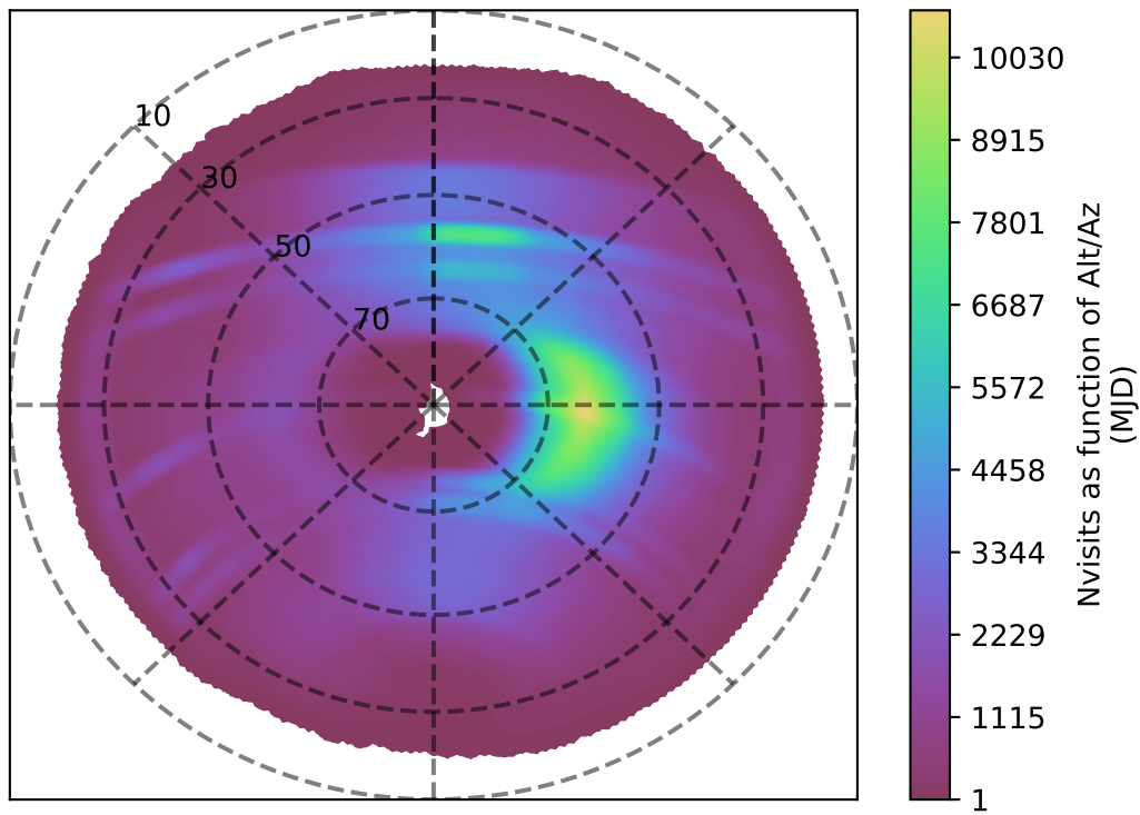
too_elab_r32_d3_gz_v3.4_10yrs all bands: Nvisits as function of Alt/Az
