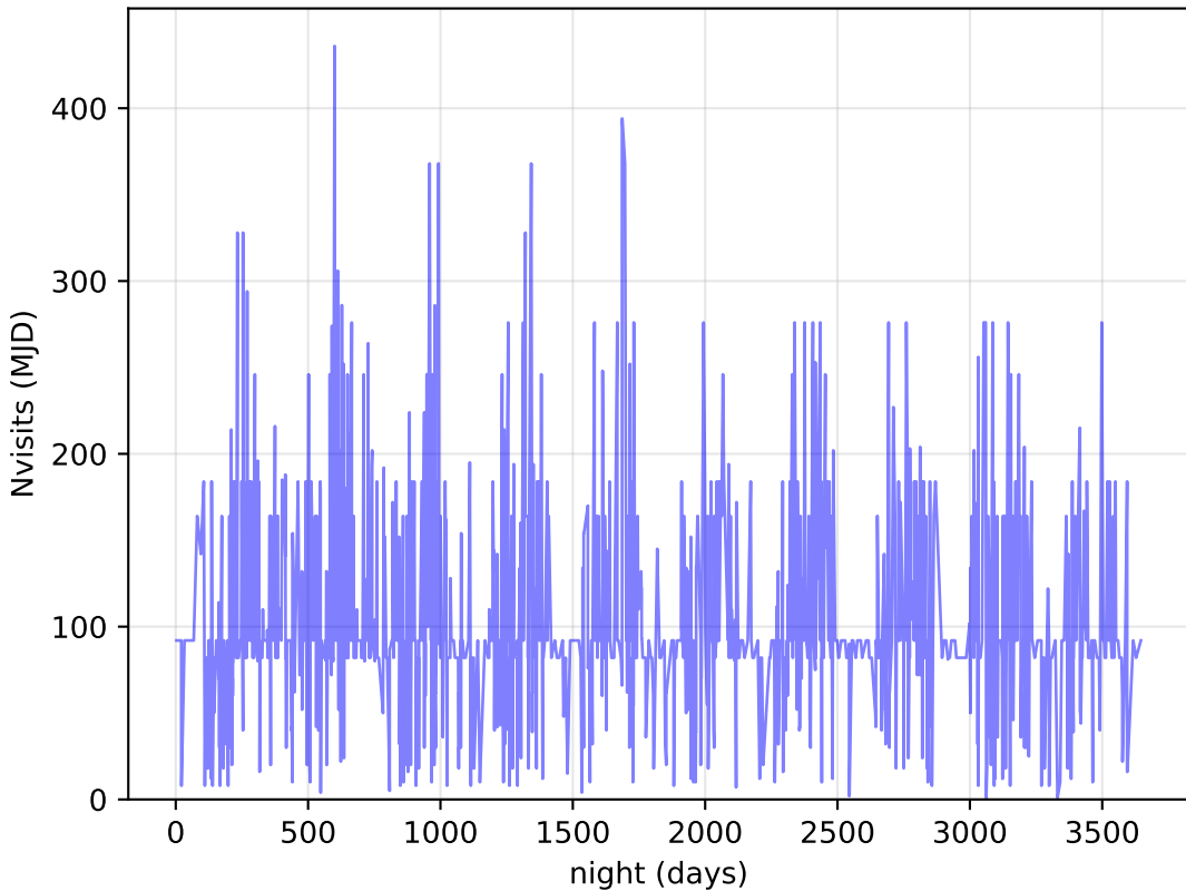
too_elab_r32_d3_gz_v3.4_10yrs DDF: Nvisits
