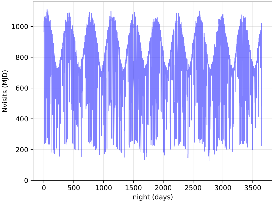
too_elab_r32_d3_gz_v3.4_10yrs All visits: Nvisits
