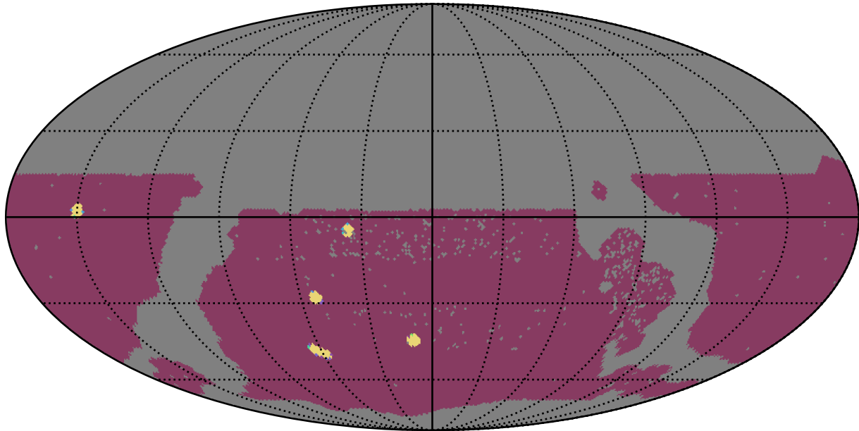
too_elab_r32_d3_gz_v3.4_10yrs WFD: NumberOfQuickRevisits
