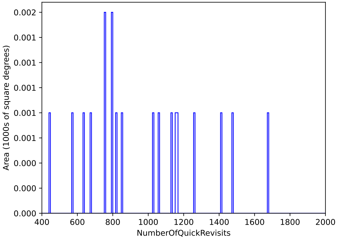
too_elab_r32_d3_gz_v3.4_10yrs WFD: NumberOfQuickRevisits
