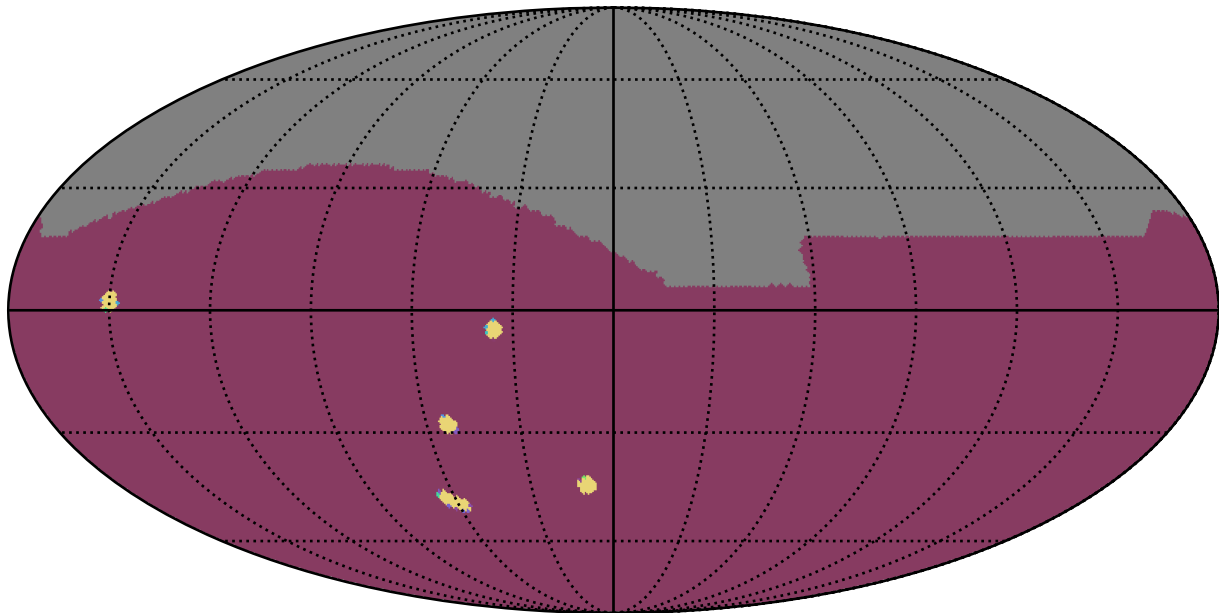
too_elab_r32_d3_gz_v3.4_10yrs All sky: NumberOfQuickRevisits
