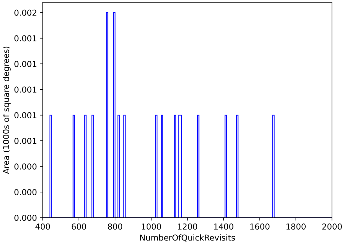
too_elab_r32_d3_gz_v3.4_10yrs All sky: NumberOfQuickRevisits
