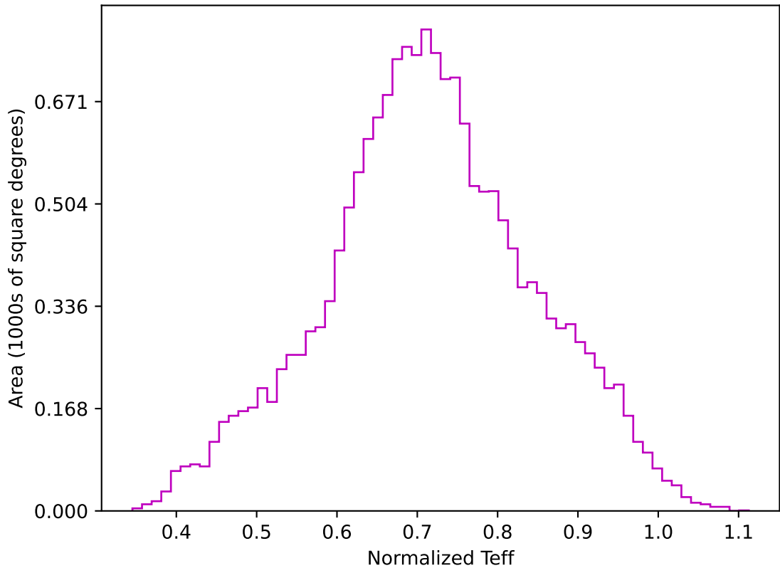
too_elab_r32_d3_gz_v3.4_10yrs WFD z band: Normalized Teff
