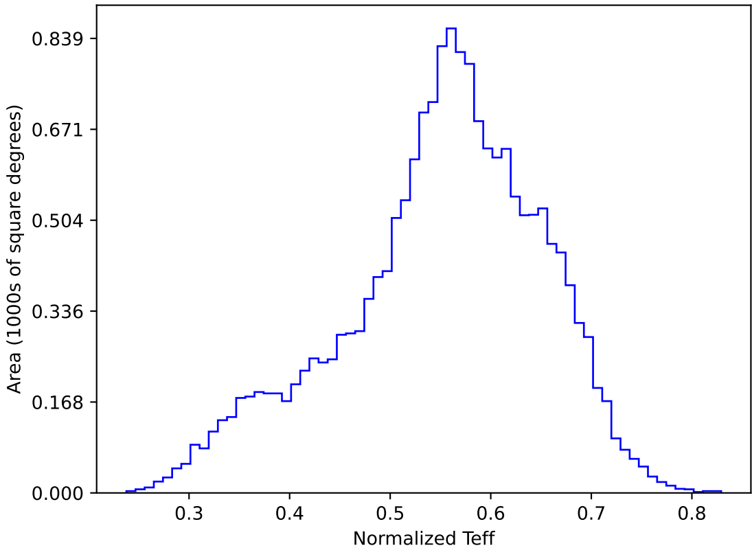
too_elab_r32_d3_gz_v3.4_10yrs WFD y band: Normalized Teff
