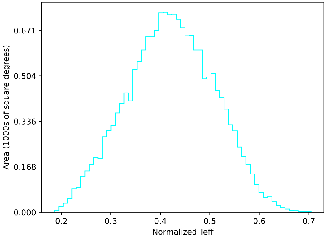
too_elab_r32_d3_gz_v3.4_10yrs WFD u band: Normalized Teff
