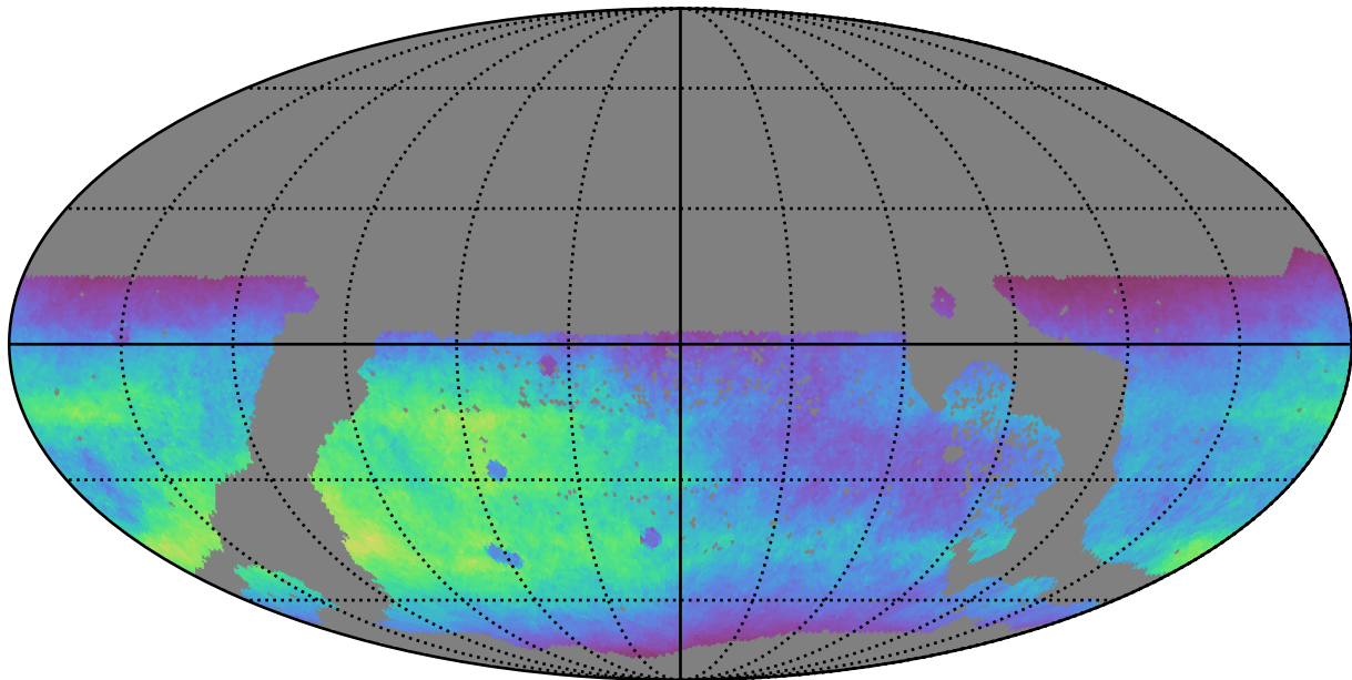
too_elab_r32_d3_gz_v3.4_10yrs WFD r band: Normalized Teff
