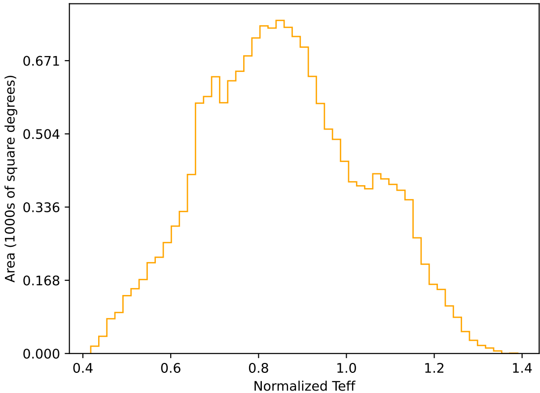
too_elab_r32_d3_gz_v3.4_10yrs WFD r band: Normalized Teff
