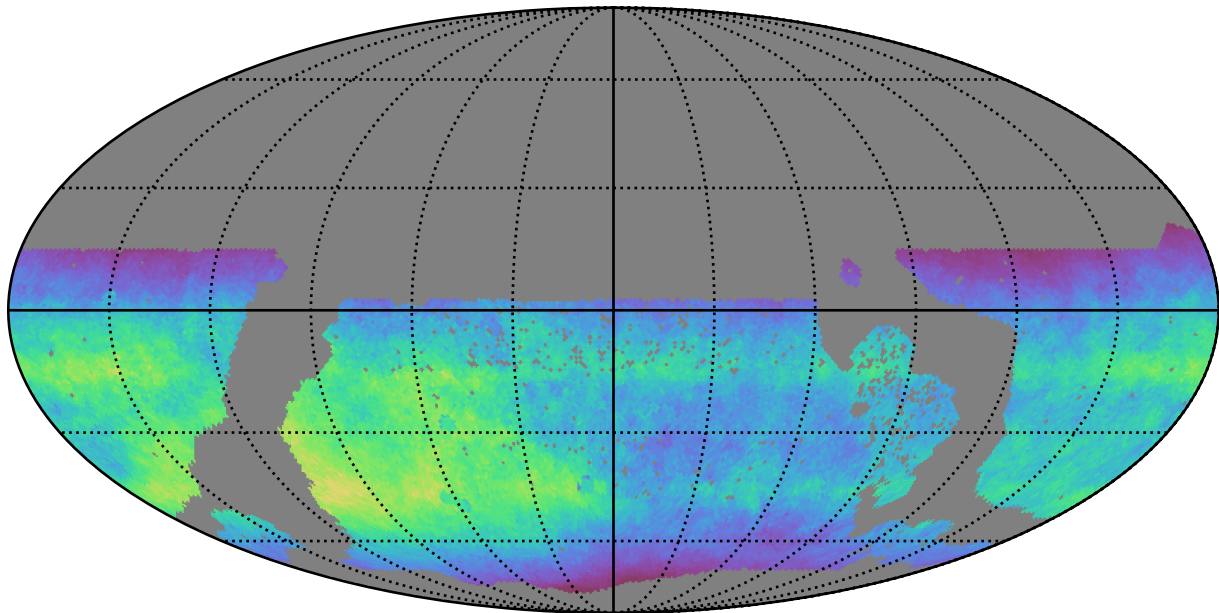
too_elab_r32_d3_gz_v3.4_10yrs WFD i band: Normalized Teff
