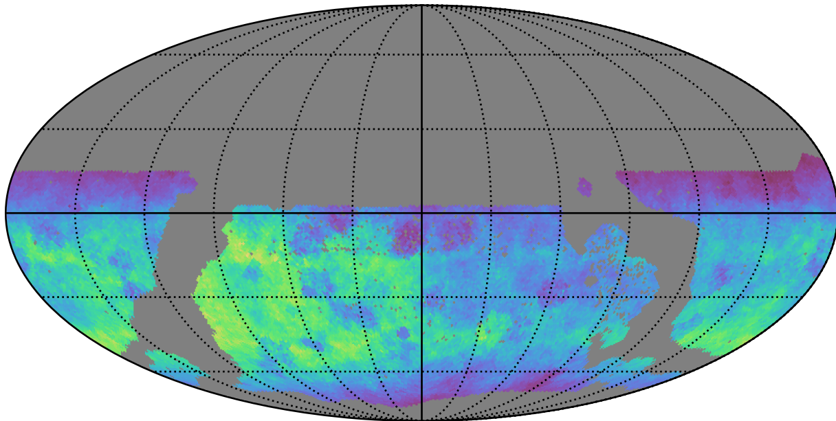
too_elab_r32_d3_gz_v3.4_10yrs WFD g band: Normalized Teff
