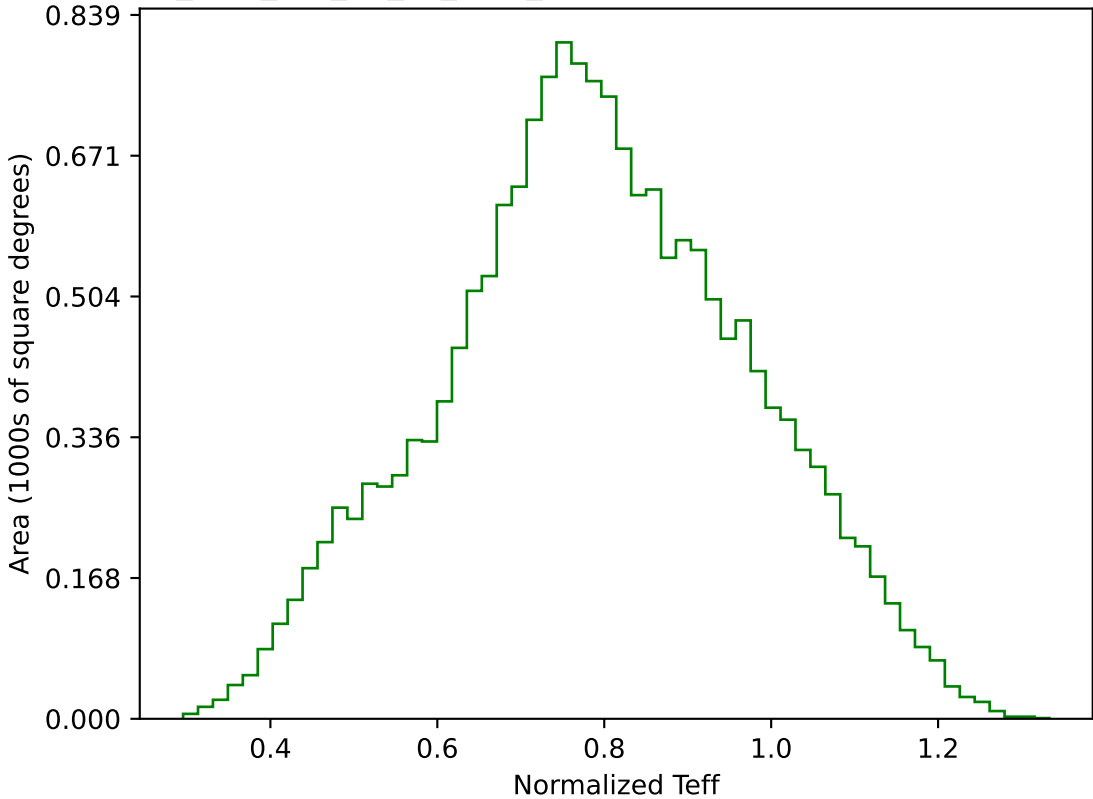
too_elab_r32_d3_gz_v3.4_10yrs WFD g band: Normalized Teff
