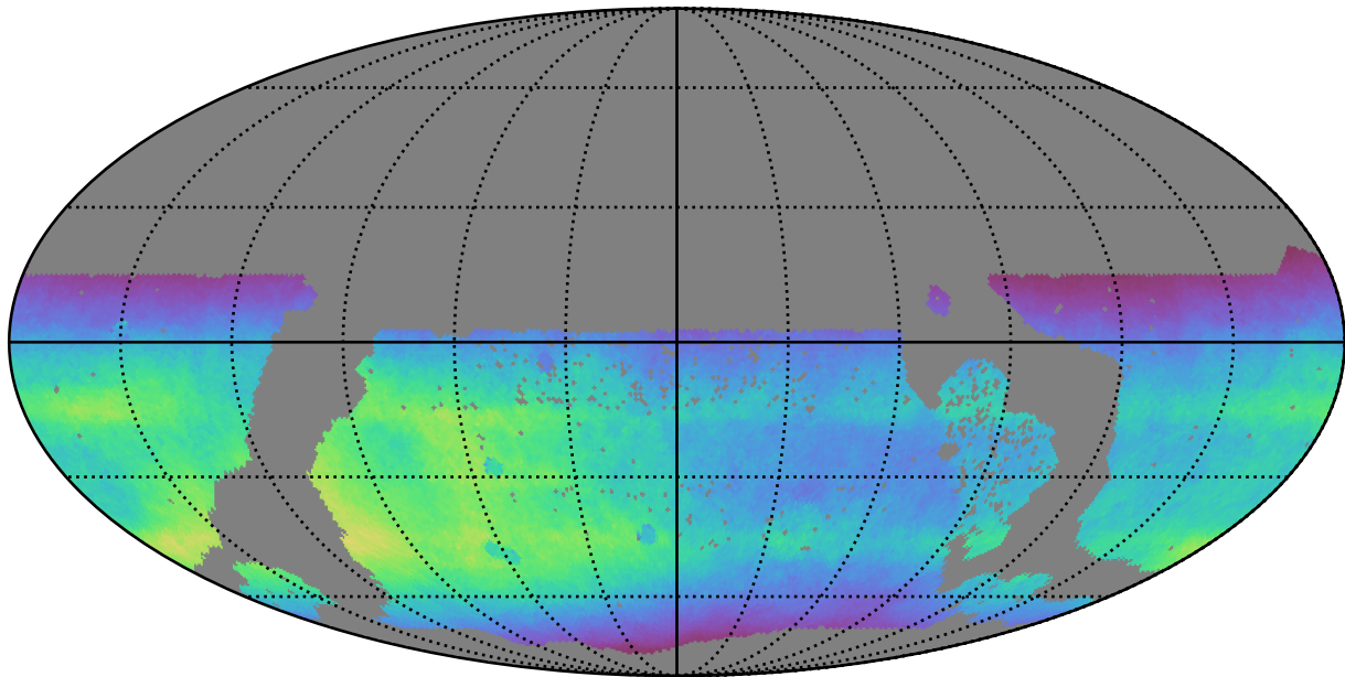
too_elab_r32_d3_gz_v3.4_10yrs WFD all bands: Normalized Teff
