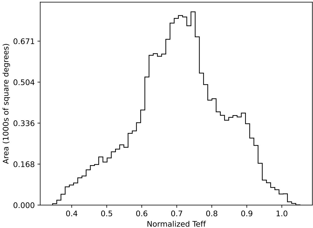
too_elab_r32_d3_gz_v3.4_10yrs WFD all bands: Normalized Teff
