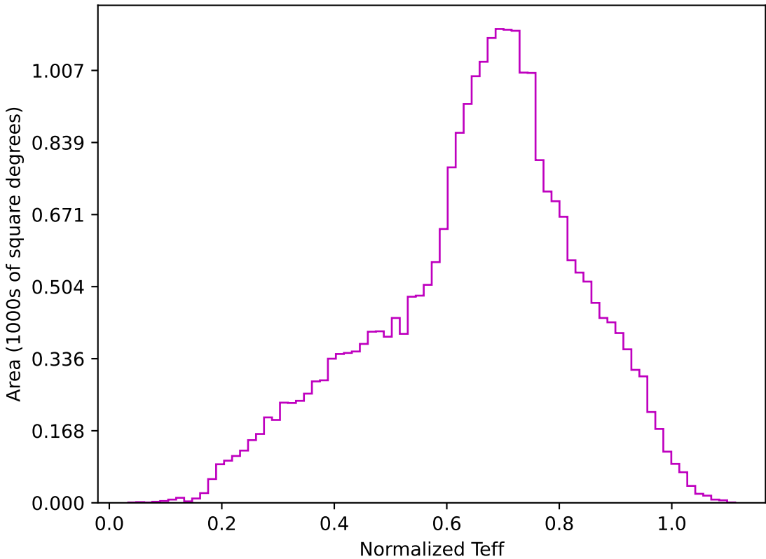
too_elab_r32_d3_gz_v3.4_10yrs All sky z band: Normalized Teff
