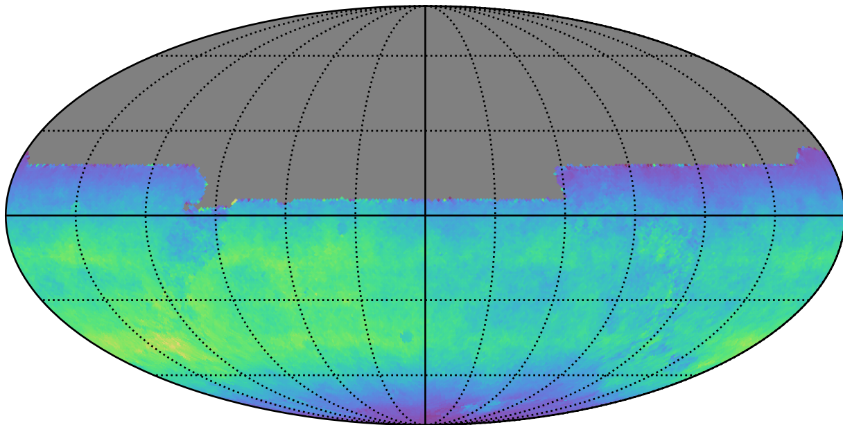
too_elab_r32_d3_gz_v3.4_10yrs All sky y band: Normalized Teff
